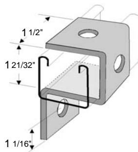
Three-Hole Cup Support
