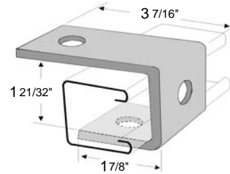
Three-Hole Suspension Clevis
