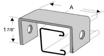
Two-Hole Clevis
