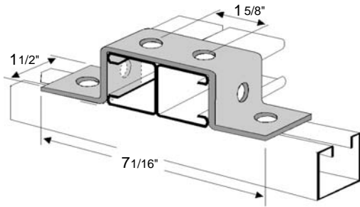
Six-Hole "U" Support
