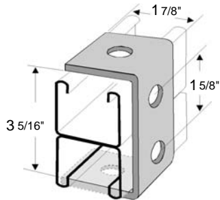
Four-Hole Clevis
