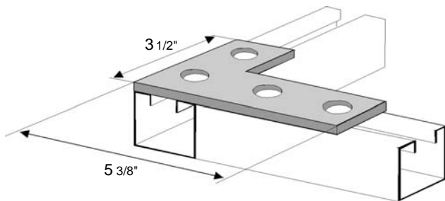
Four-Hole Corner Plate FP604
