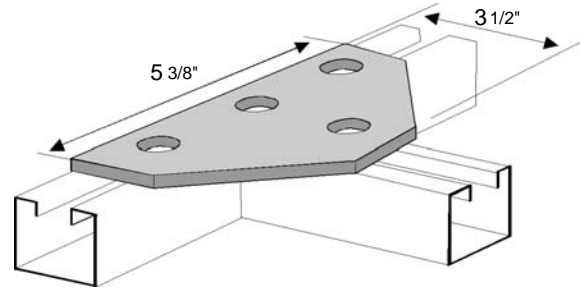
Four-Hole Tee Gusset FP601
