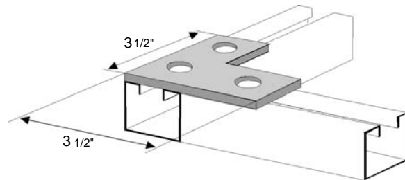
Three-Hole Corner Plate FP500
